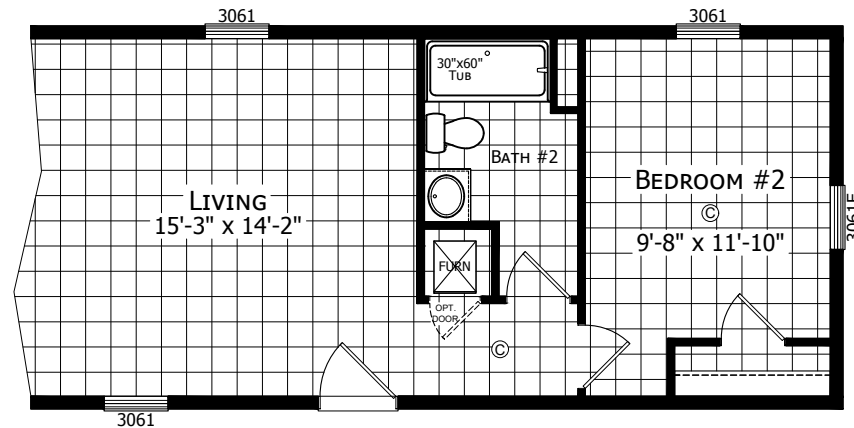
2 BEDROOM OPTION
