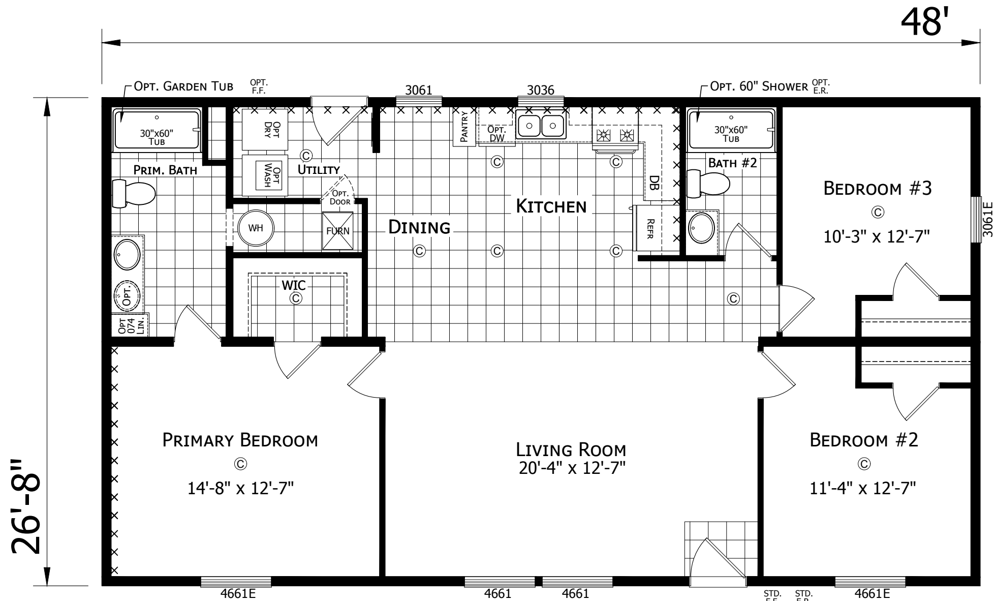
112APB-2848H32024 3 BEDROOM 2 BATH 48'-0" x 26'-8" 1280 SQ. FT. TOTAL
