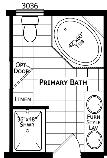
OPTIONAL PRIMARY BATH
