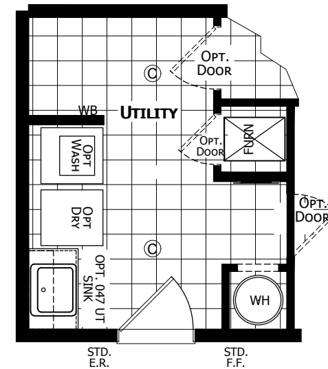
OPTIONAL DOOR LOCATION REQUIRES PATIO DOOR IN DINING ROOM
